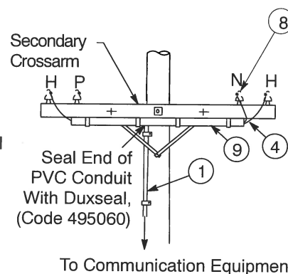
Figure 3 Installation With Extended Rack Secondary
