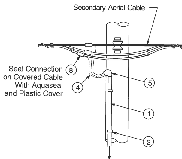
Figure 2 Installation With Aerial Cable Secondary
