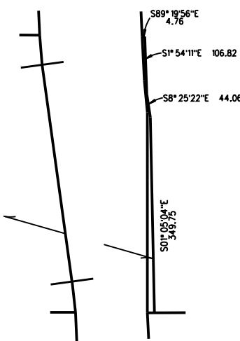
DETAIL NO SCALE
