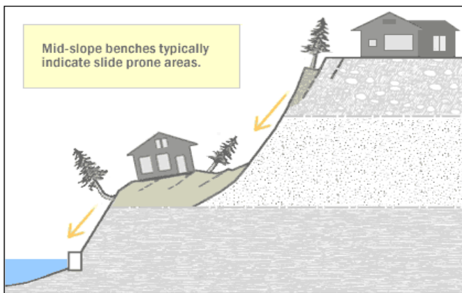
Figure 10-3. Bench Slide
