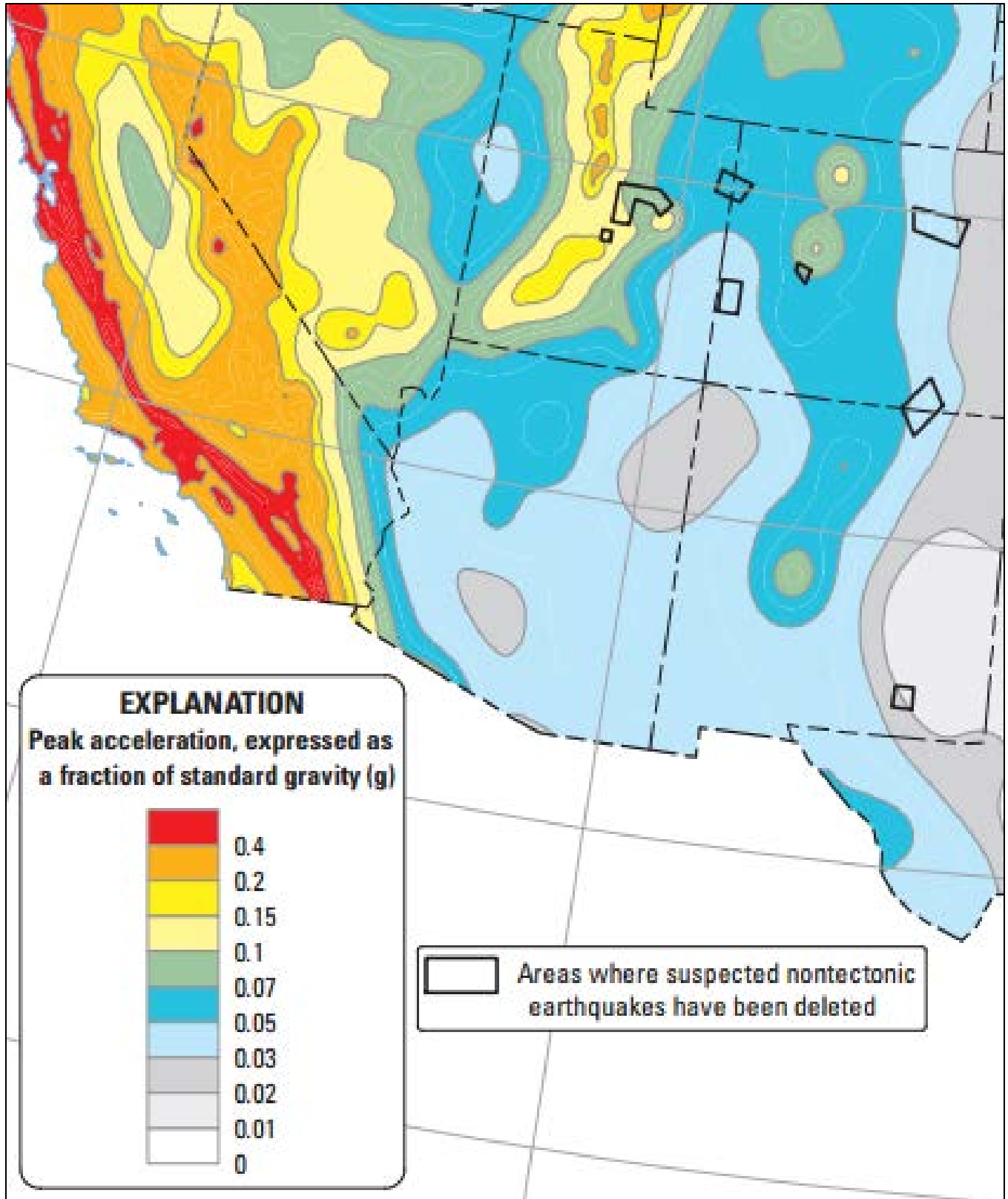
Figure 8-11. Peak Ground Acceleration with 10-percent Probability of Exceedance in 50 Years
