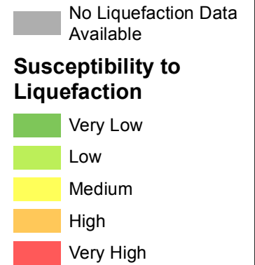
Figure 8-10. Liquefaction Susceptibility
