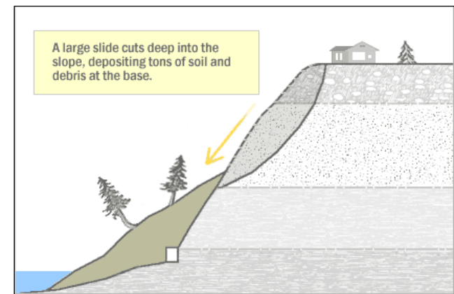
Figure 10-4. Large Slide
