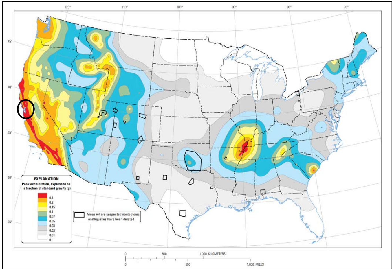
Figure 8-1. Peak Acceleration (%g) with 10% Probability of Exceedance in 50 Years
