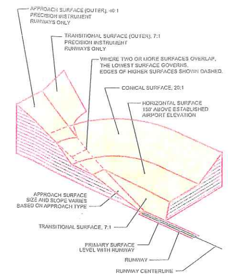
Isometric diagram of Part 77, Paragraph 77.25 Civil Airport Imaginary Surfaces
